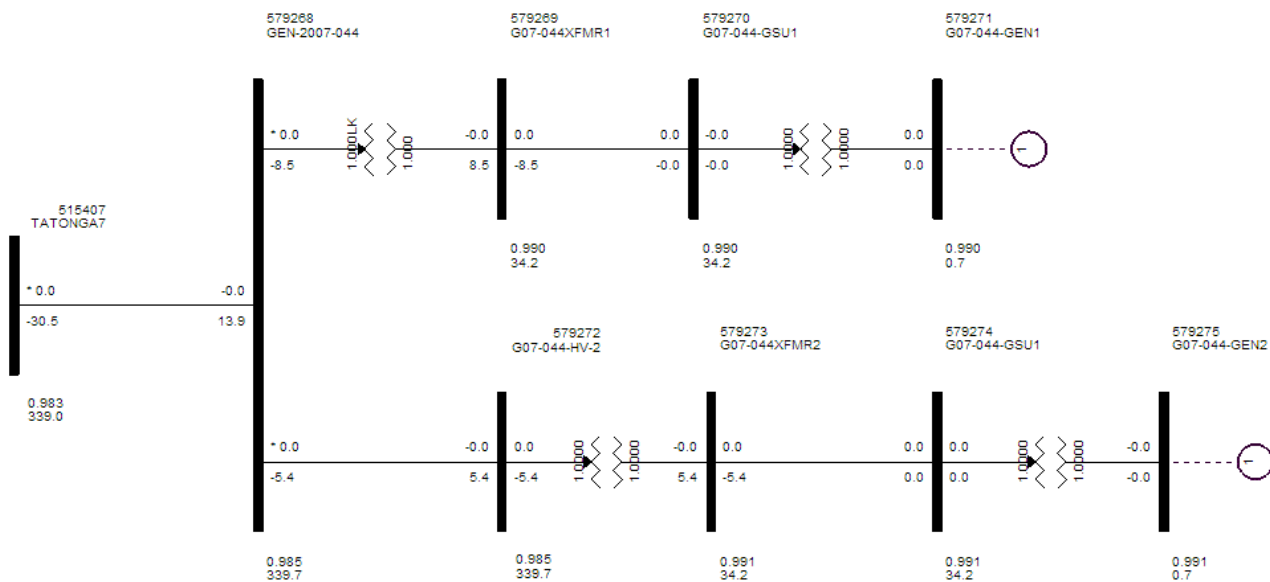
Figure IV-1: GEN-2007-044 with generators and capacitors turned off and no shunt reactors
