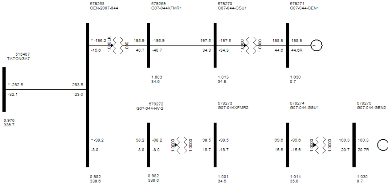
Figure II-1: GEN-2007-044 One-line Diagram
