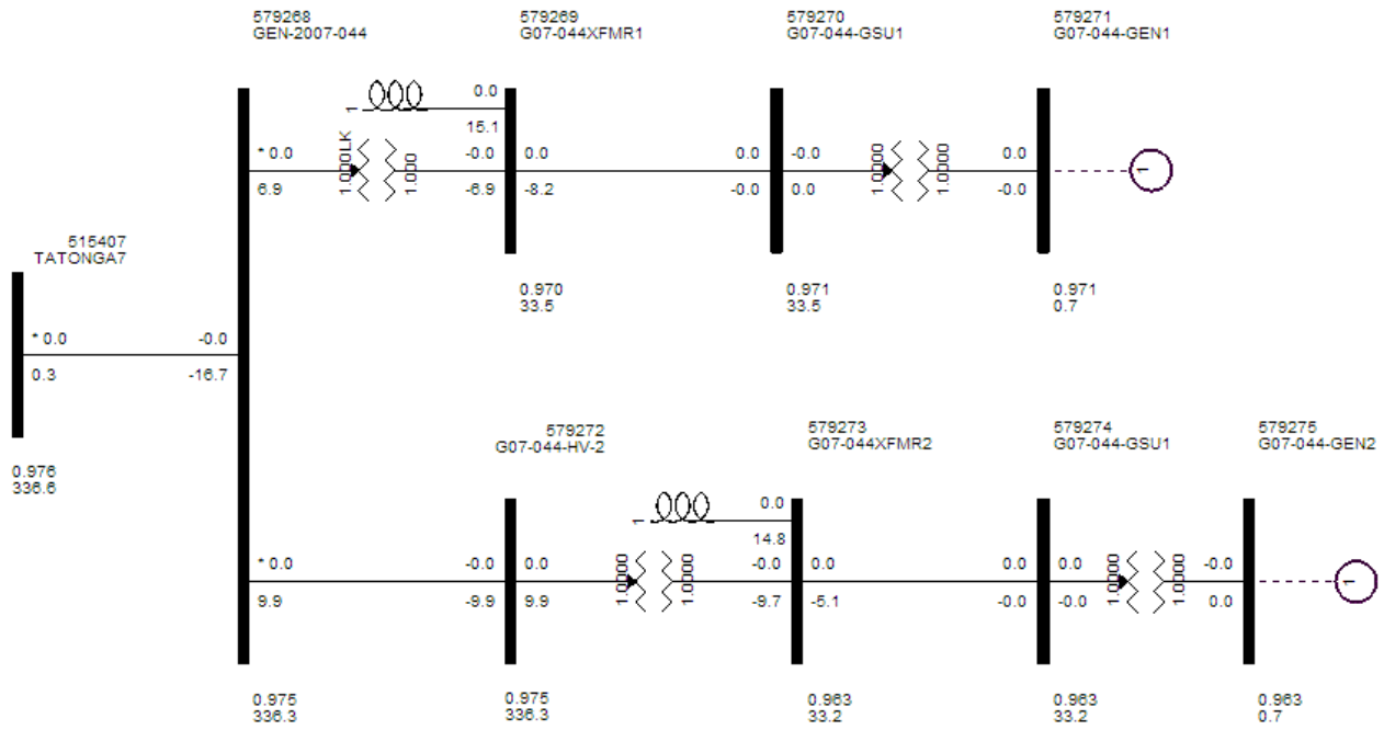
Figure IV-2: GEN-2007-044 with generators and capacitors turned off and shunt reactors added
